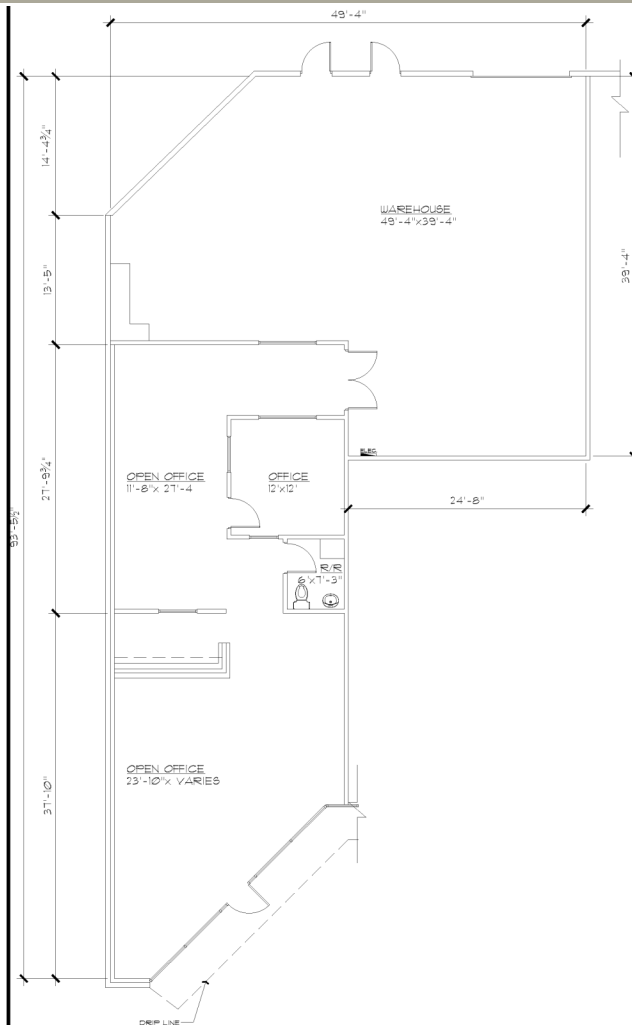
01 AS-BUILT FLOOR PLAN SUITE 408 - SUITE 3,041 S.F. SCALE: GRAPHIC
