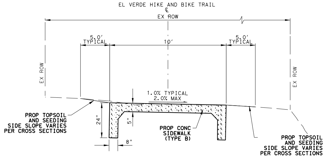
EL VERDE HIKE & BIKE TRAIL TYPICAL SECTION (SIDEWALK TYPE B) STA 10+00.00 TO STA 18+00.00 STA 42+00.00 TO STA 54+61.99
