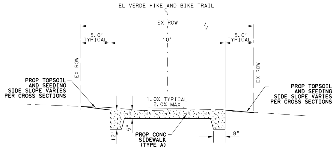
EL VERDE HIKE & BIKE TRAIL TYPICAL SECTION (SIDEWALK TYPE A) STA 18+00.00 TO STA 42+00.00
